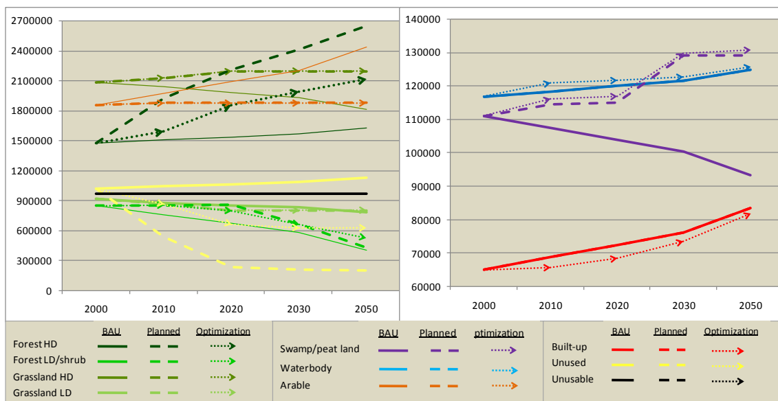
Figure 4.2 Land use change in the BAU, Planned and Optimum scenarios (Note: Y-axes are area, unit: km 2 )
