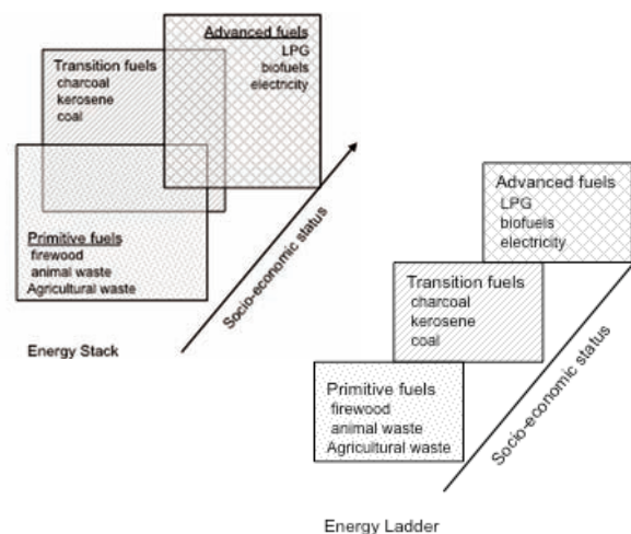
Fig. 2.1. The energy ladder and energy stack models
